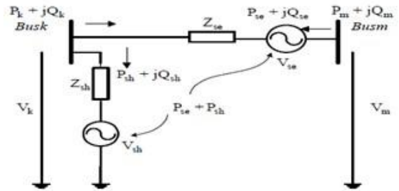
Figure 7: voltage source model of UPFC
