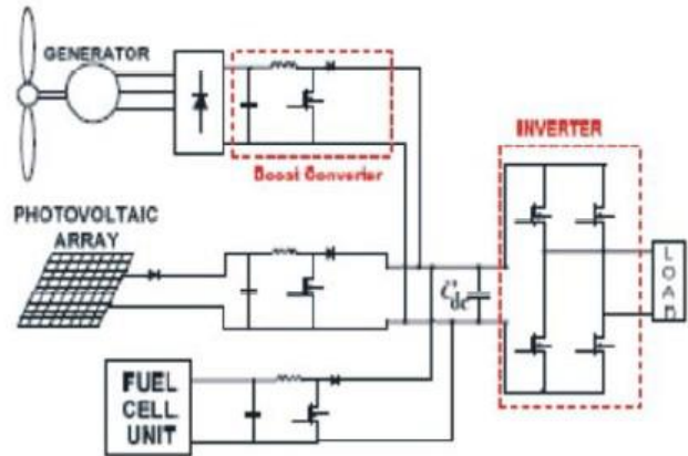
Figure 14: Hybrid system with multi-connected boost converter
