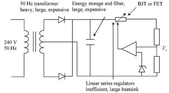
Figure 9: Practical linear series regulator circuit
