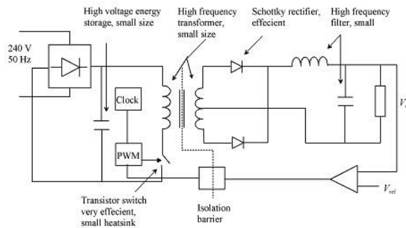
Figure 10: Practical circuit of switch mode regulator
